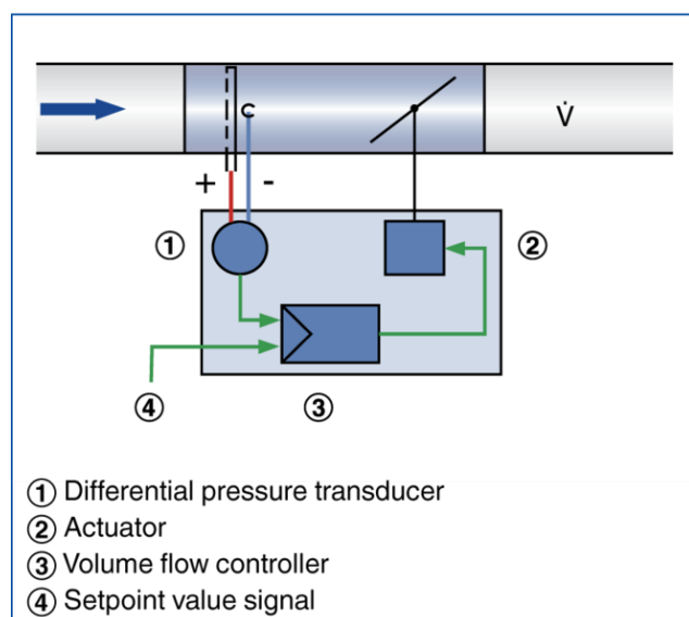
Compact controllers LMV-D3-MP and LMV-D3-MP-F
